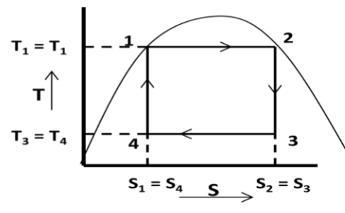
(T-s diagram)
